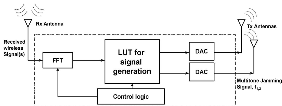
Multitone Jammer Kit Block Diagram
